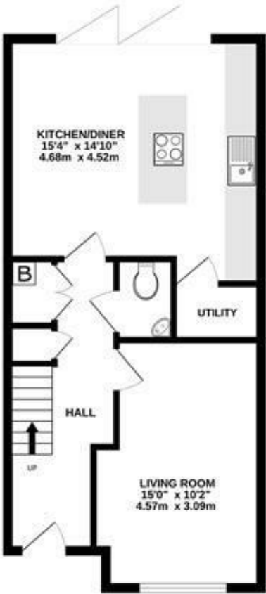
GROUND FLOOR 496 sq.ft. (46.1 sq.m.) approx.
